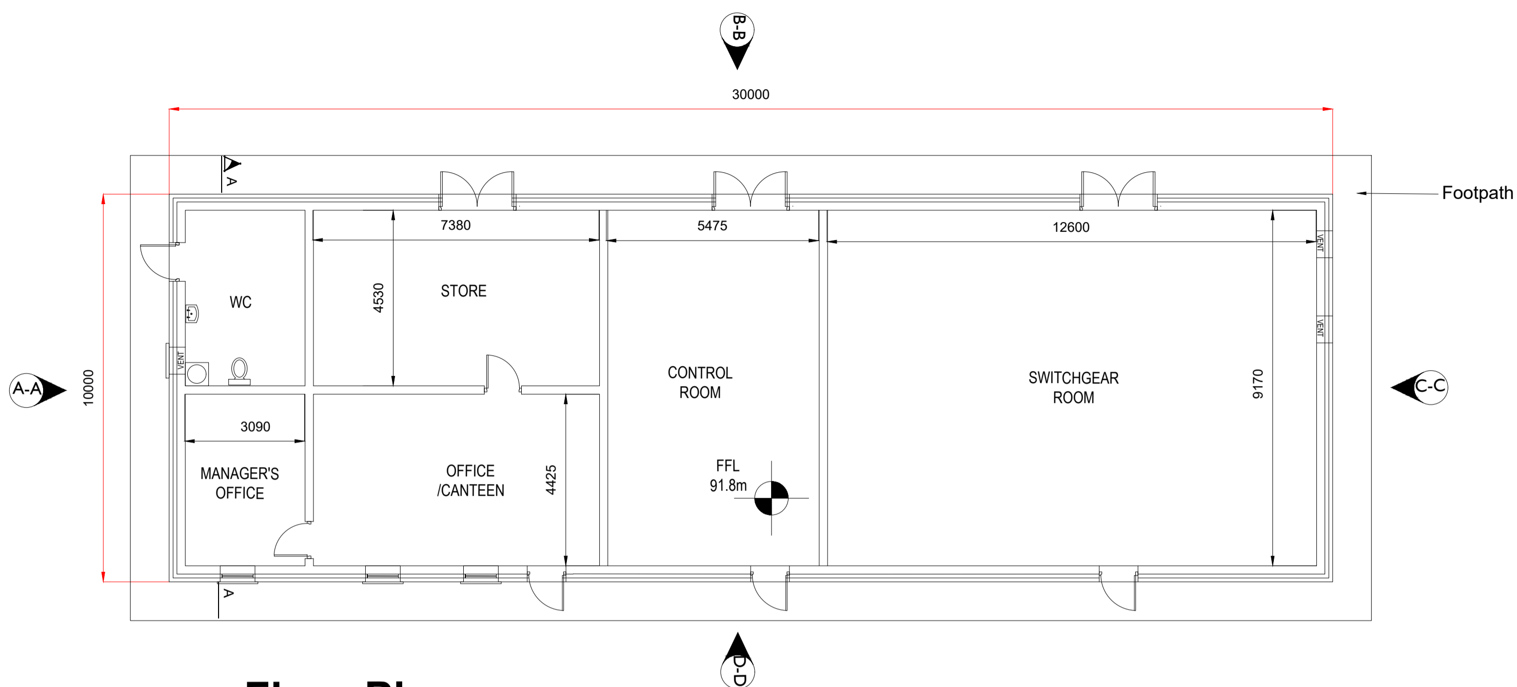
Floor Plan Scale 1:100
